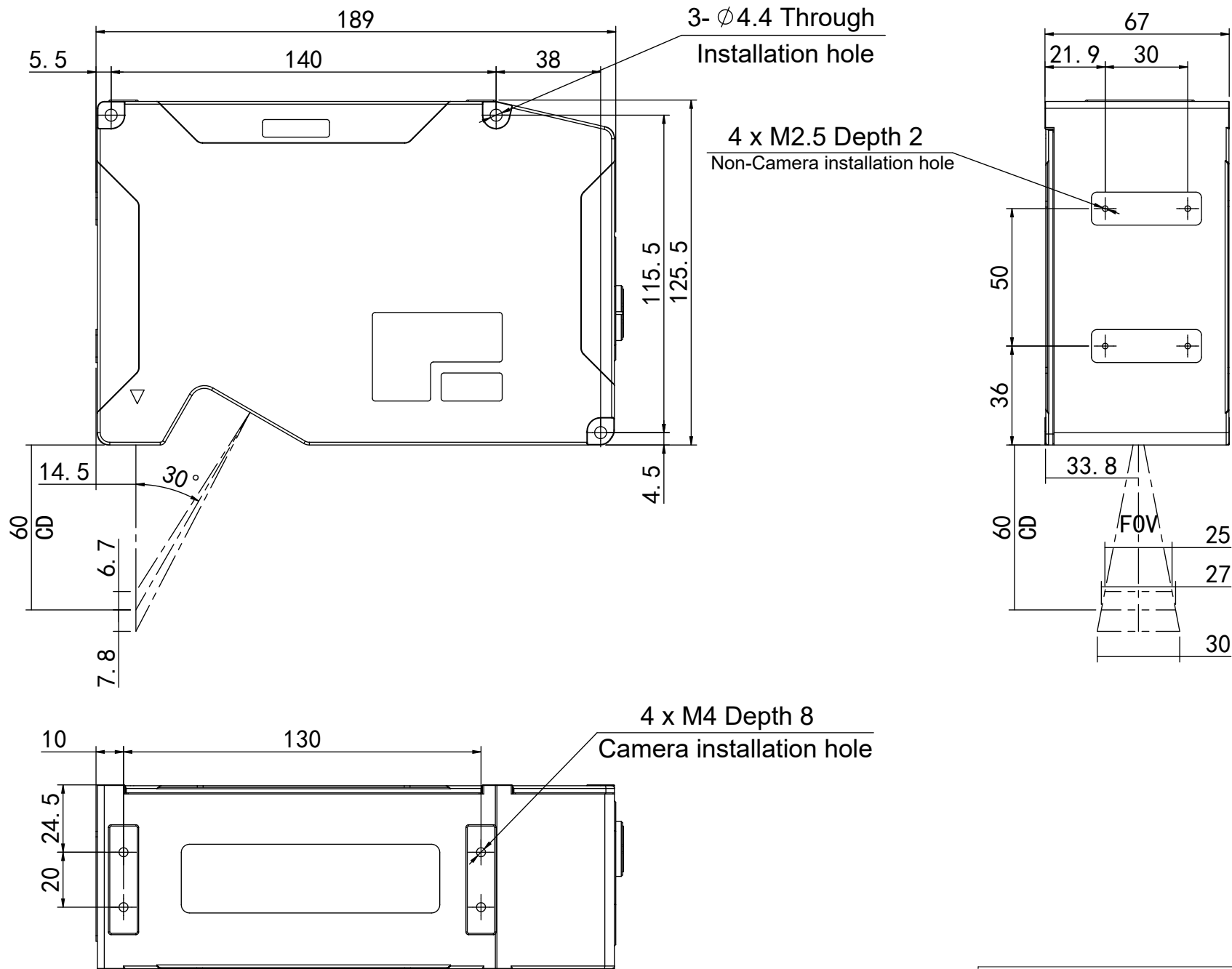
SR9061 Installation Diagram
